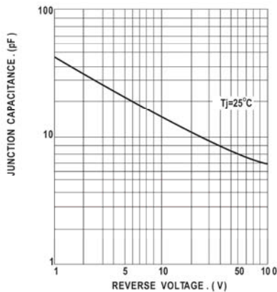
FIG . 2-TYPICAL JUNCTION CAPACITANCE
